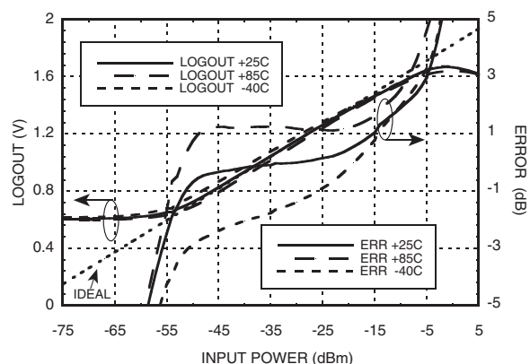
LOGOUT Voltage & Error vs. Input Power, F_{in} = 3500 MHz
