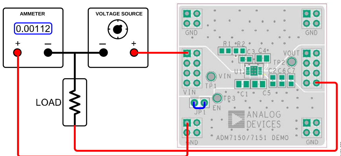
Figure 6. Ground Current Measurement, LFCSP
