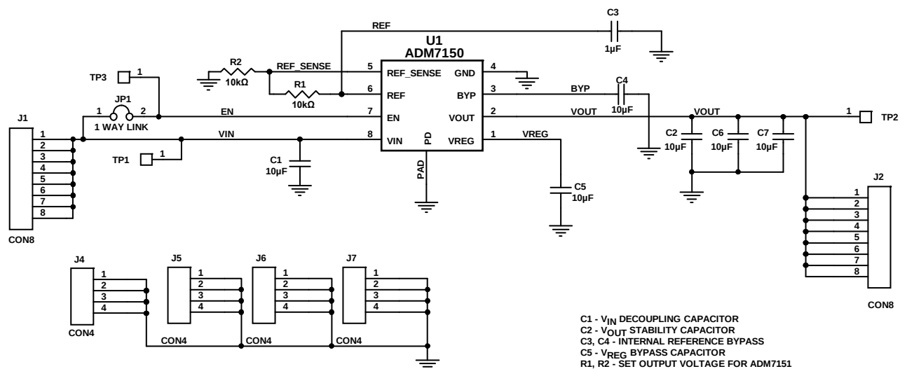
Figure 8. Evaluation Board Schematic
