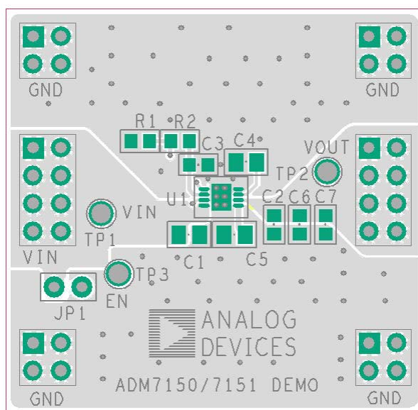
Figure 1. ADM7150CP-EVALZ/ADM7151CP-02-EVALZ LFCSP Evaluation Board
