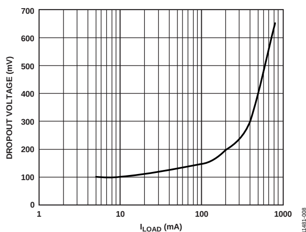
Figure 5. Dropout Voltage vs. Load Current
