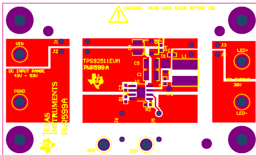
Figure 12. Top Layer and Top Overlay (Top View)
