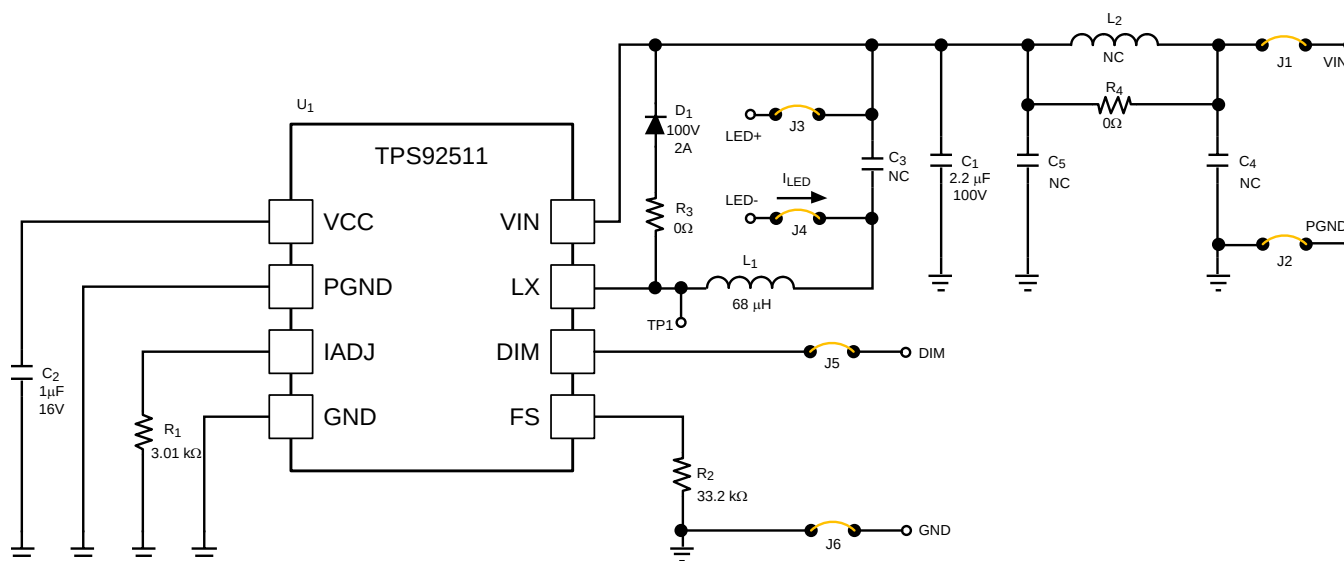
Figure 1. TPS92511EVM Schematic
