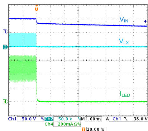
Figure 9. Shut-down Waveform
