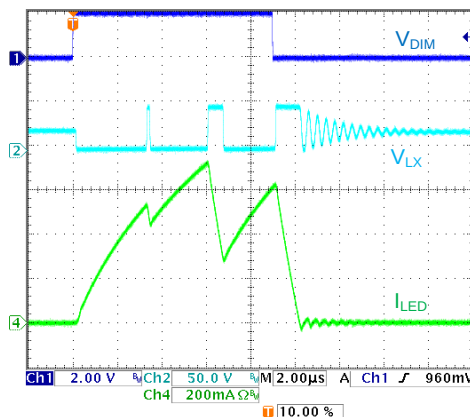
Figure 6. PWM Dimming, f_{\text{PWM}} = 240 \text{ Hz} , Pulse Width = 9 \mu\text{s}
