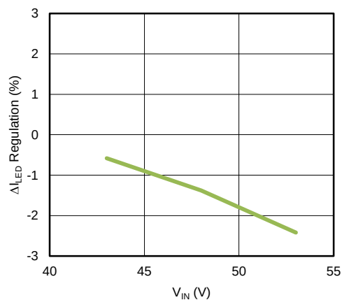
Figure 3. Line Regulation
