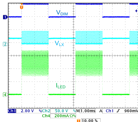
Figure 5. PWM Dimming, f_{\text{PWM}} = 240 \text{ Hz} , Duty Cycle = 50%
