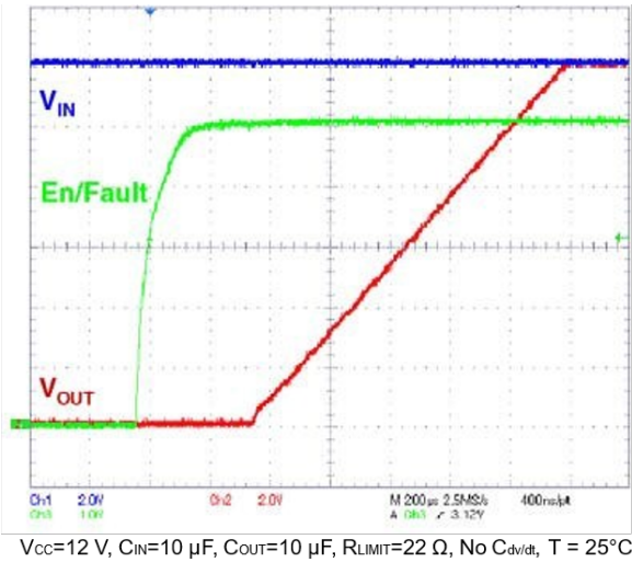
Figure 15. V_{OUT} ramp-up vs. enable
