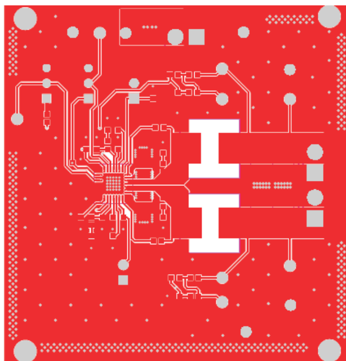
Figure 3. Top Layer
