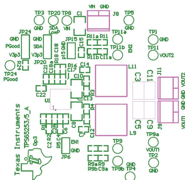
Figure 2. Part Placement
