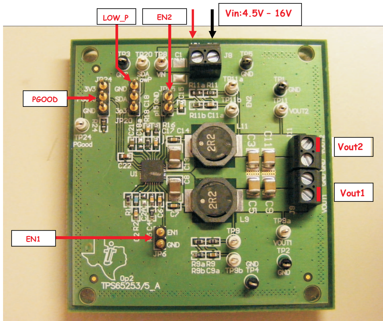
Figure 7. Headers Description and Jumper Placement
