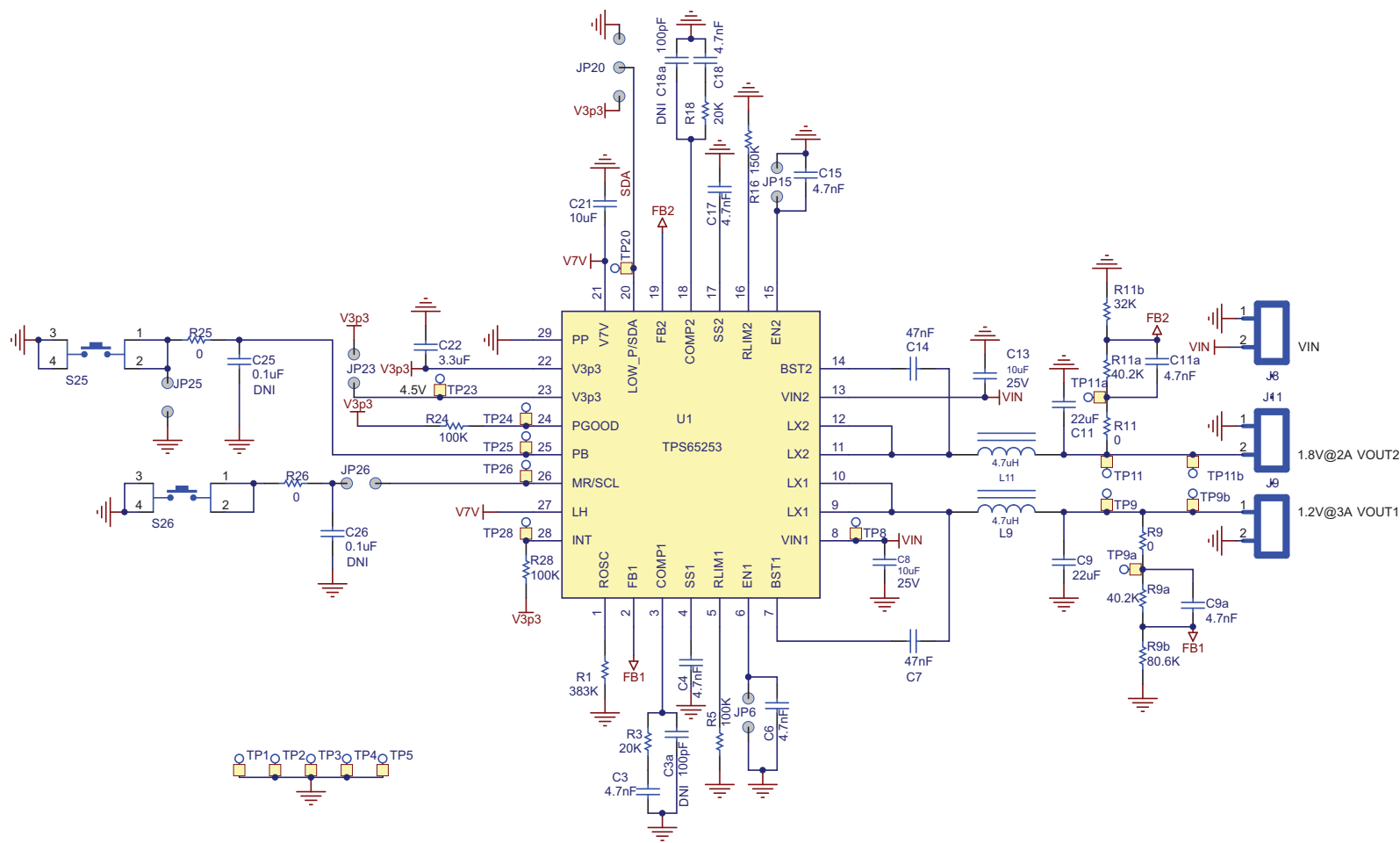
Figure 1. TPS65253 Schematic
