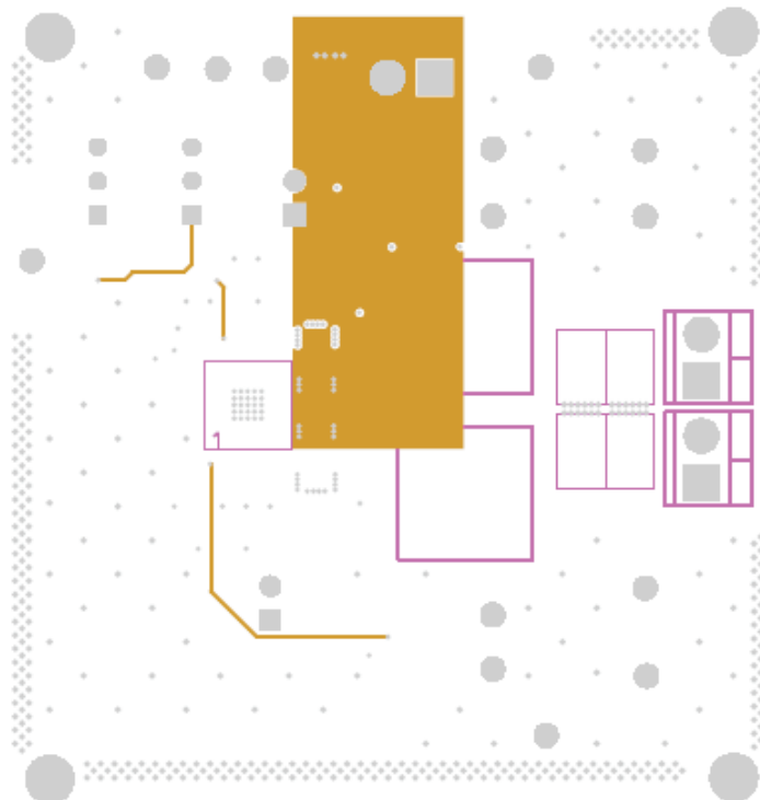
Figure 5. Mid-Layer 2
