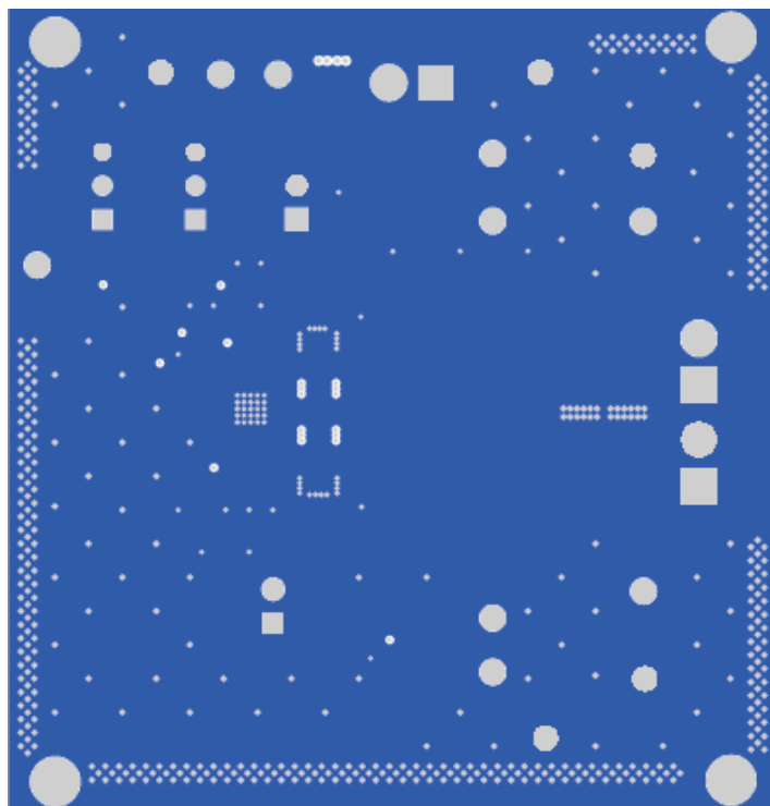
Figure 6. Bottom Layer
