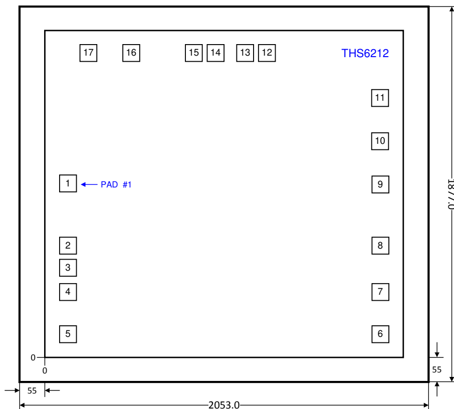
Figure 89. Die Dimensions
