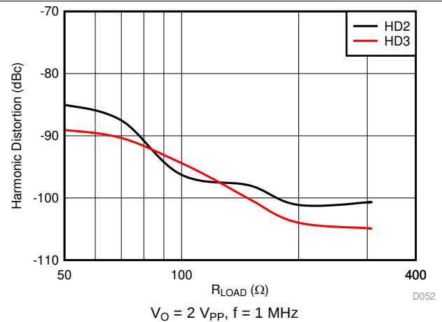
Figure 52. Harmonic Distortion vs Load Resistance
