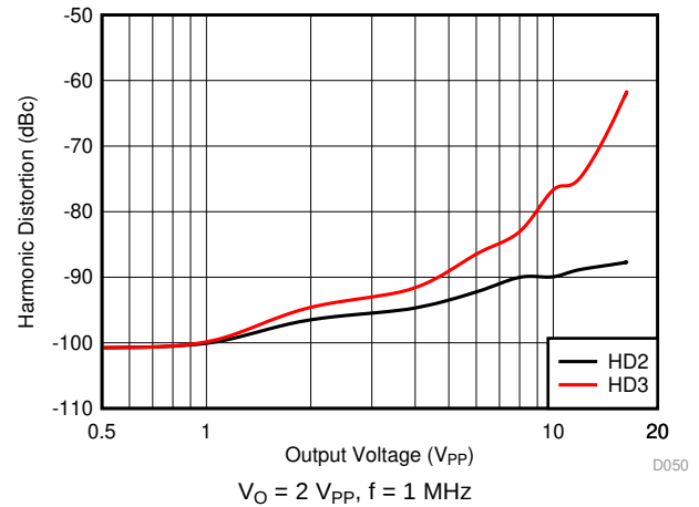
Figure 50. Harmonic Distortion vs Output Voltage
