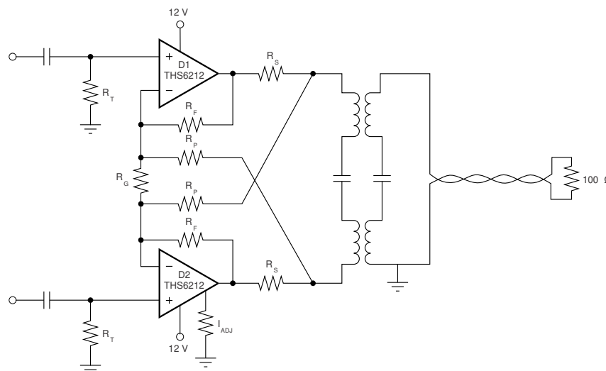
Typical Line-Driver Circuit Using the THS6212
