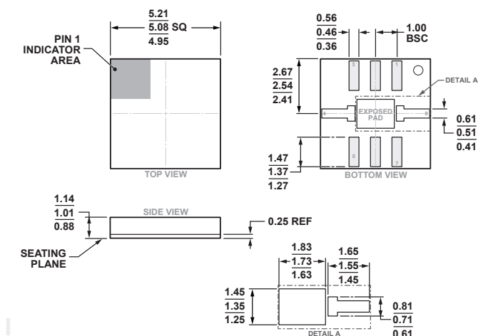
8-Terminal Chip Array Small Outline No Lead Cavity [LGA_CAV] 5.08 mm x 5.08 mm Body and 1.01 mm Package Height (CE-8-1) Dimensions shown in millimeters
