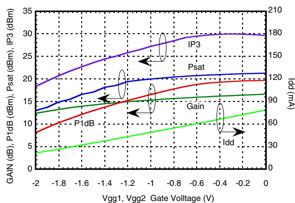
Gain, Power, Output IP3 & Idd vs. Gate Voltage @ 12 GHz
