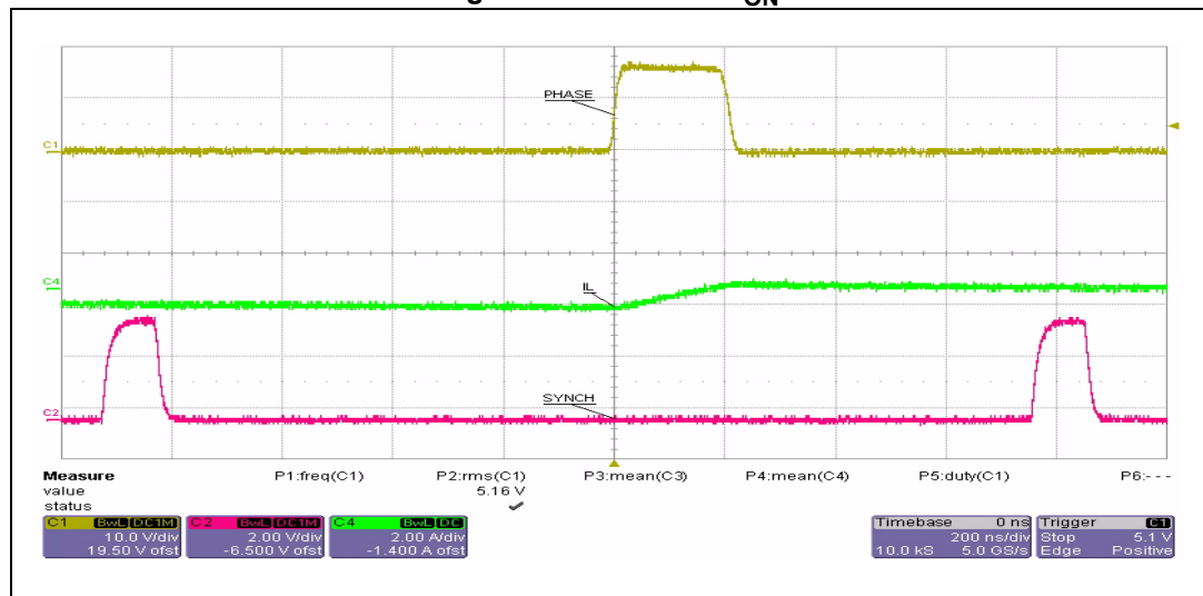
Figure 12. Minimum T_{ON}
