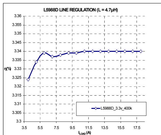
Figure 38. Line regulation
