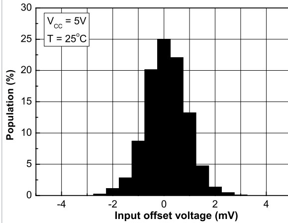
Figure 11. Input offset voltage distribution, V_{CC} = 5\text{ V}
