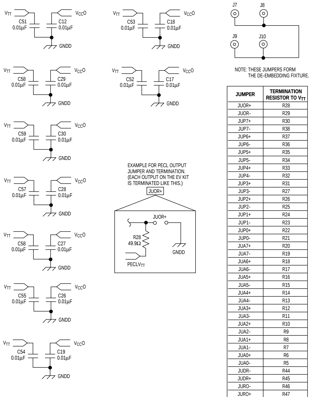
Figure 6. MAX104/MAX106/MAX108 EV Kits Schematic (continued)
