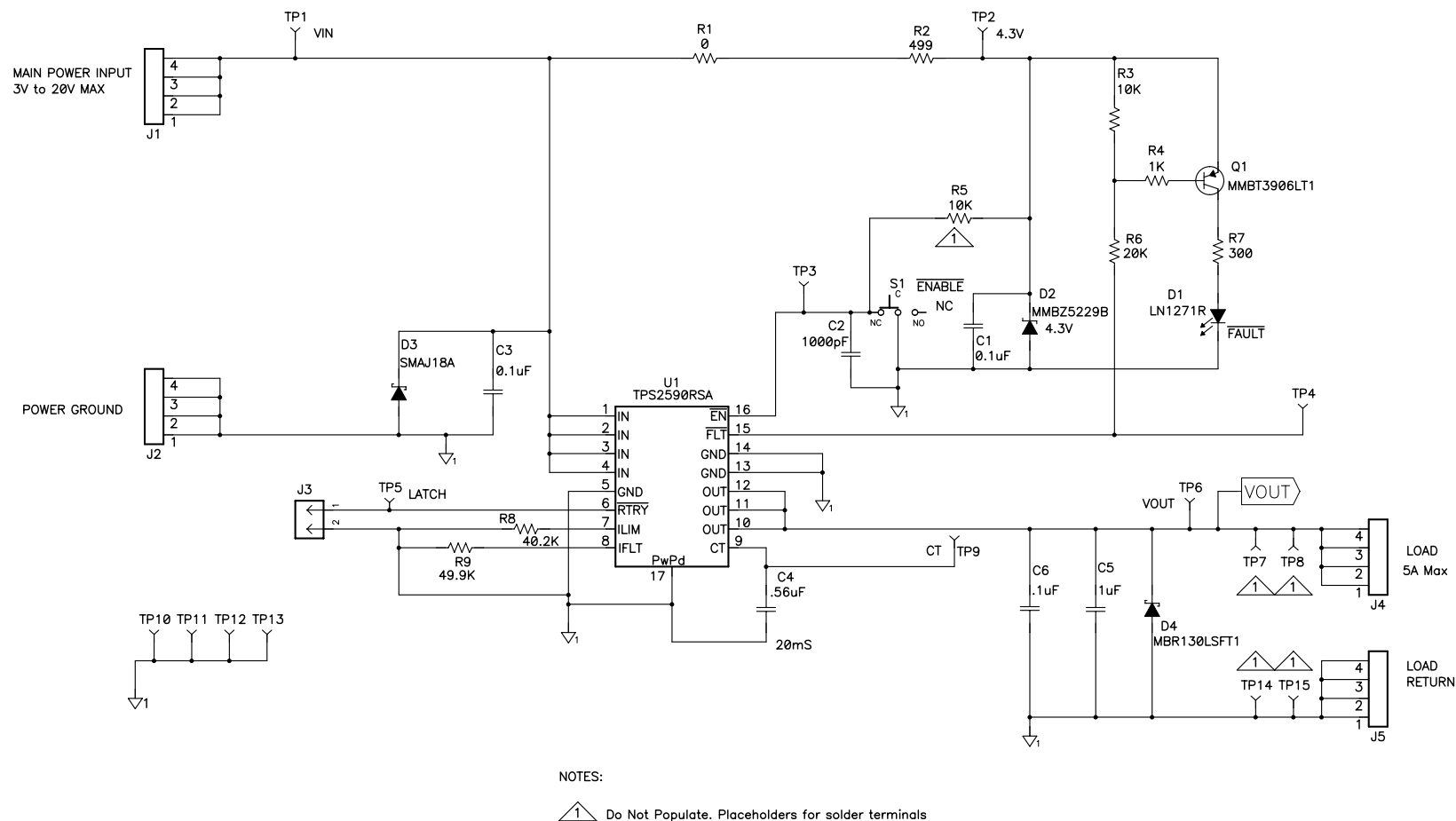
Figure 2. TPS2590EVM Schematic
