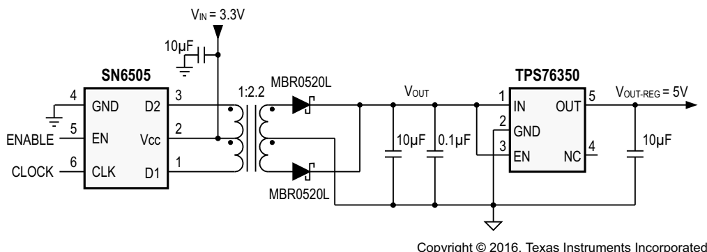
Figure 42. Typical Application Schematic
