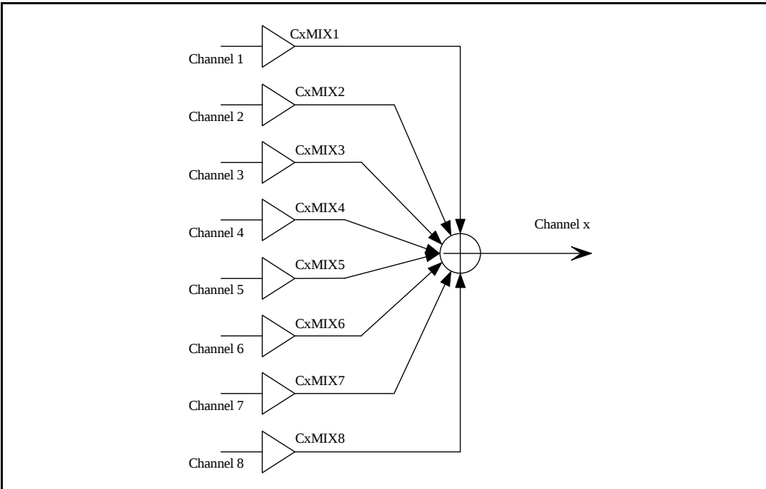
Figure 8. Channel mixer
