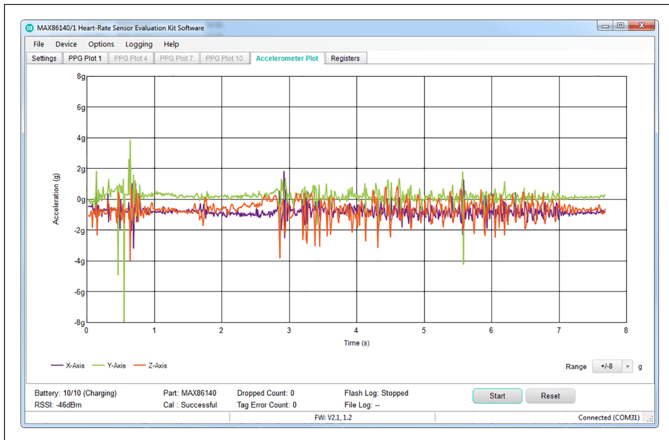
Figure 16. MAX86140 EVSYS GUI (Accelerometer Plots)
