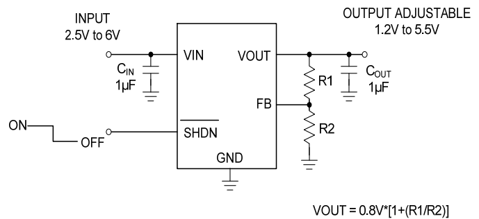
Figure 3 – LX8213-00 Adjustable Output Application Schematic
