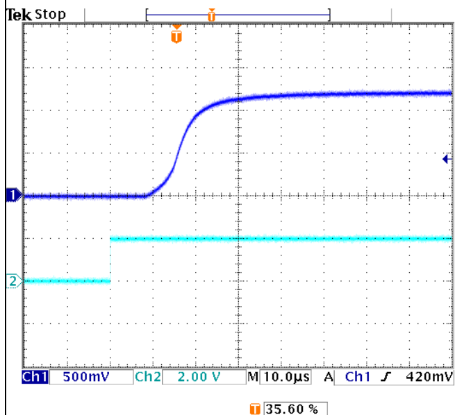
Channel 1 – 1.2V Output at No Load Channel 2 – \overline{\text{SHDN}} 0V to 2V
