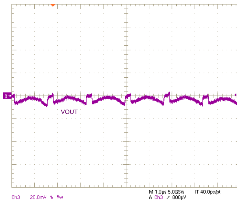
Figure 10. Output Voltage Ripple; V_{IN} = 12 V, V_{OUT} = 1.8 V, I_{OUT} = 20 A
