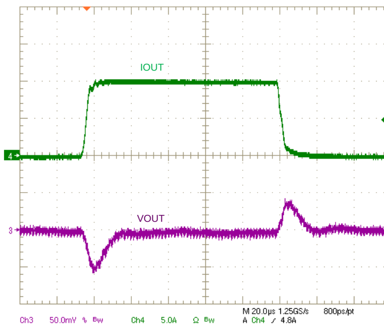
Figure 9. Load Transient Response; V_{IN} = 12 V, V_{OUT} = 1.8 V, 0 A to 10 A at 2 A/ \mu s
