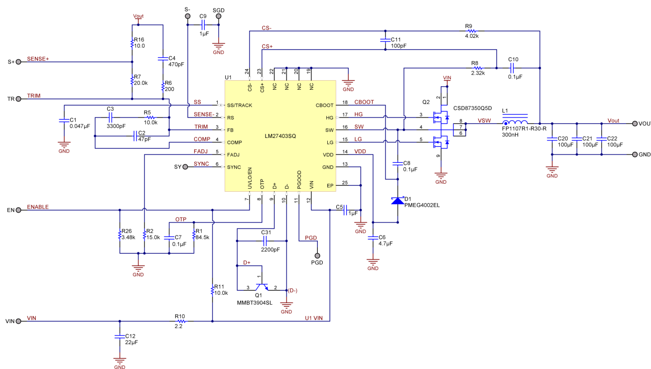
Figure 19. Module Schematic
