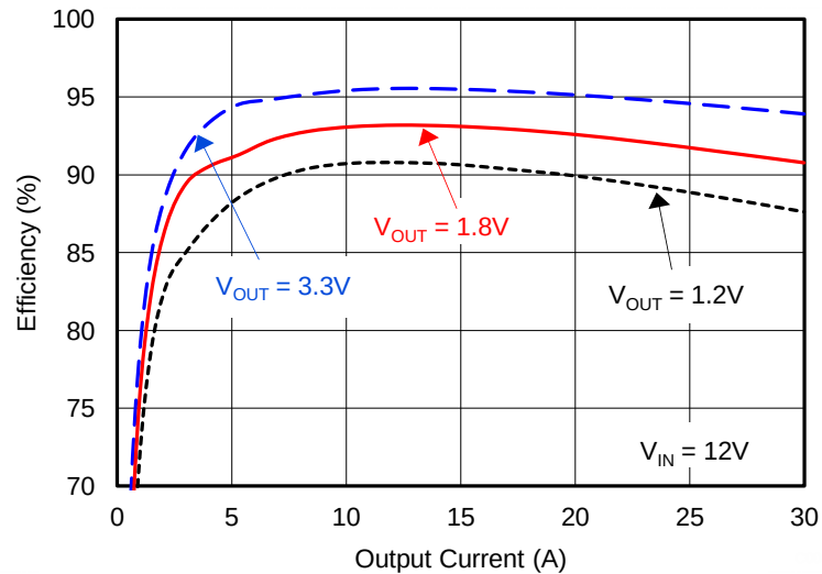
Figure 5. Efficiency
