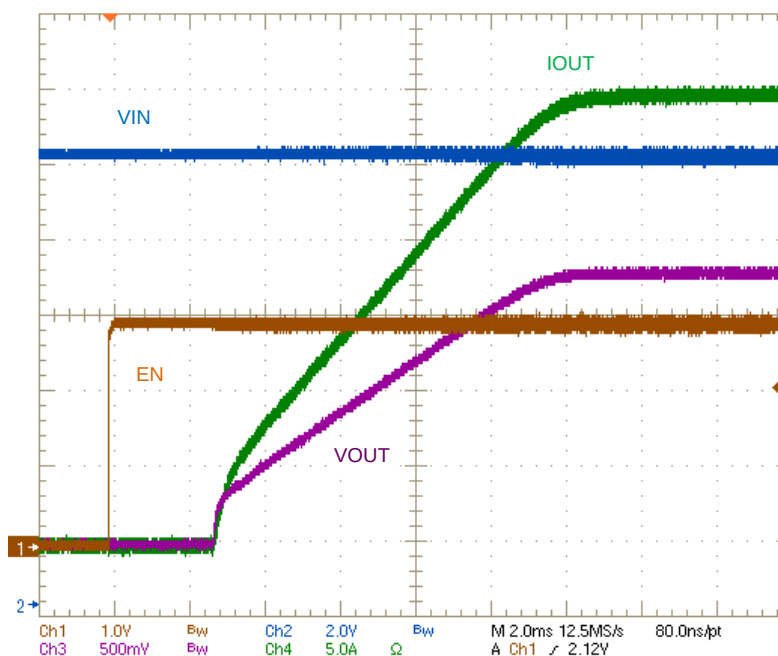
Figure 13. Startup with EN Stepped to 3 V; V_{IN} = 12\text{ V} , V_{OUT} = 1.8\text{ V} , 30-A Resistive Load
