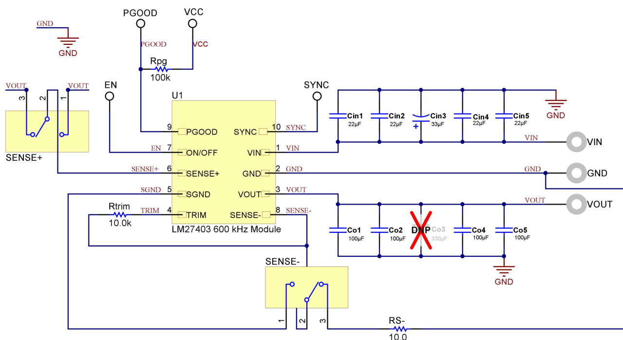
Figure 20. Motherboard Schematic
