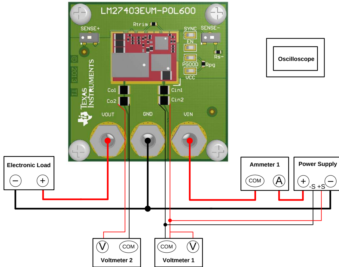
Figure 4. Connection Diagram
