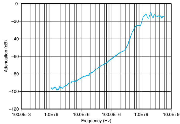
Figure 3. Crosstalk
