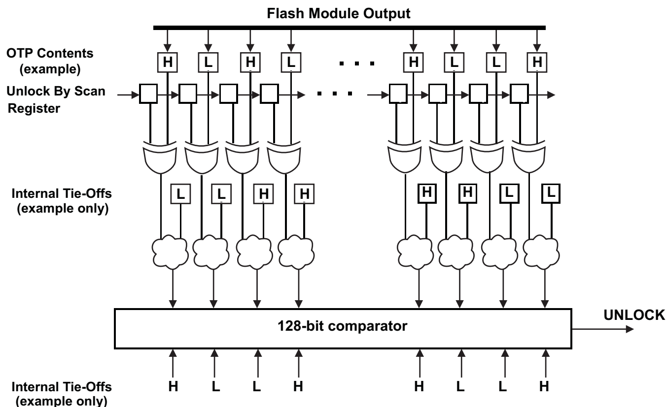
Figure 6-22. AJSM Unlock
