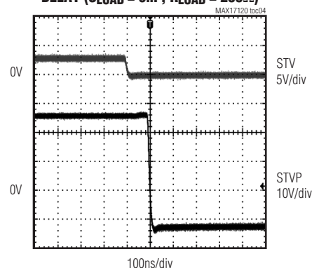
STV FALLING EDGE PROPAGATION DELAY ( C_{LOAD} = 5nF , R_{LOAD} = 200\Omega )
