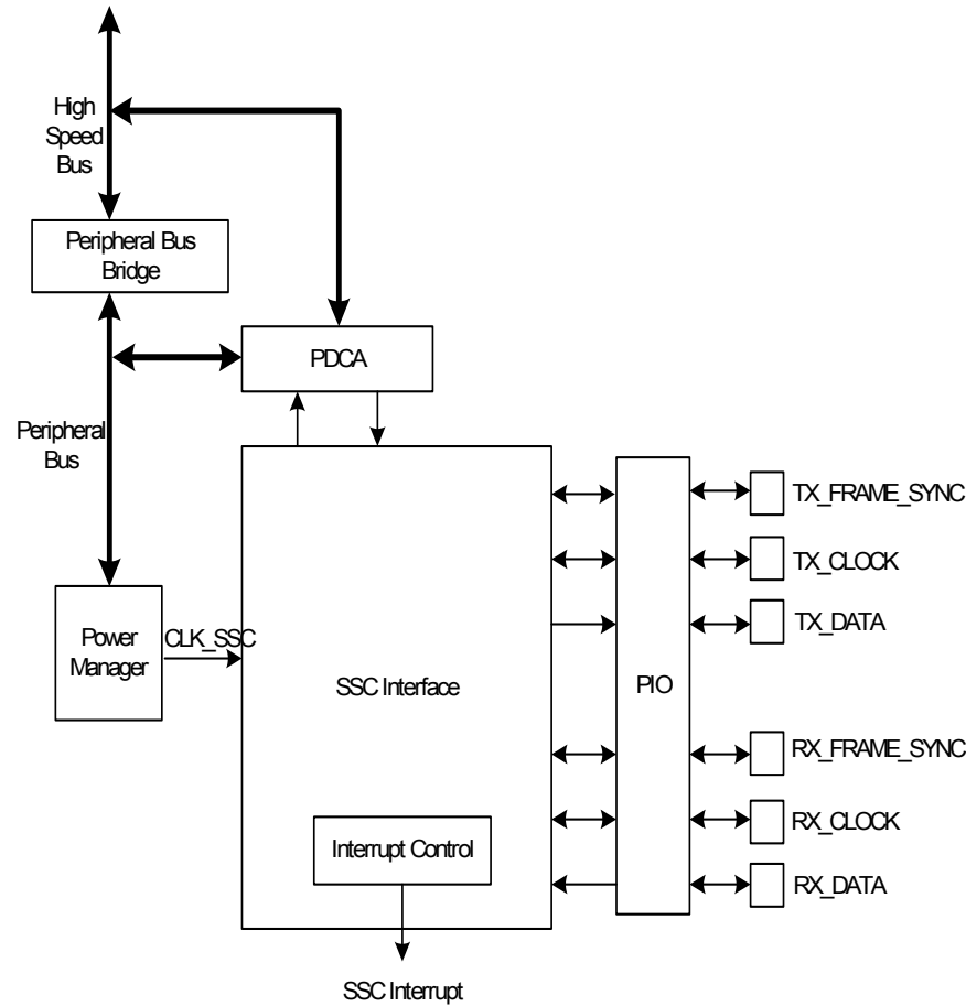
Figure 23-1. Block Diagram
