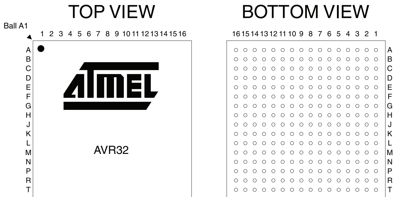
Figure 3-2. 256 CTBGA Pinout
