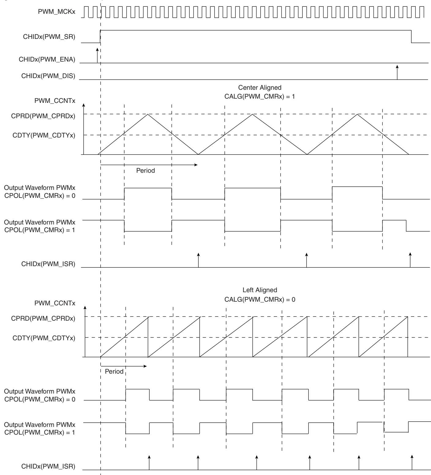
Figure 34-5. Waveform Properties
