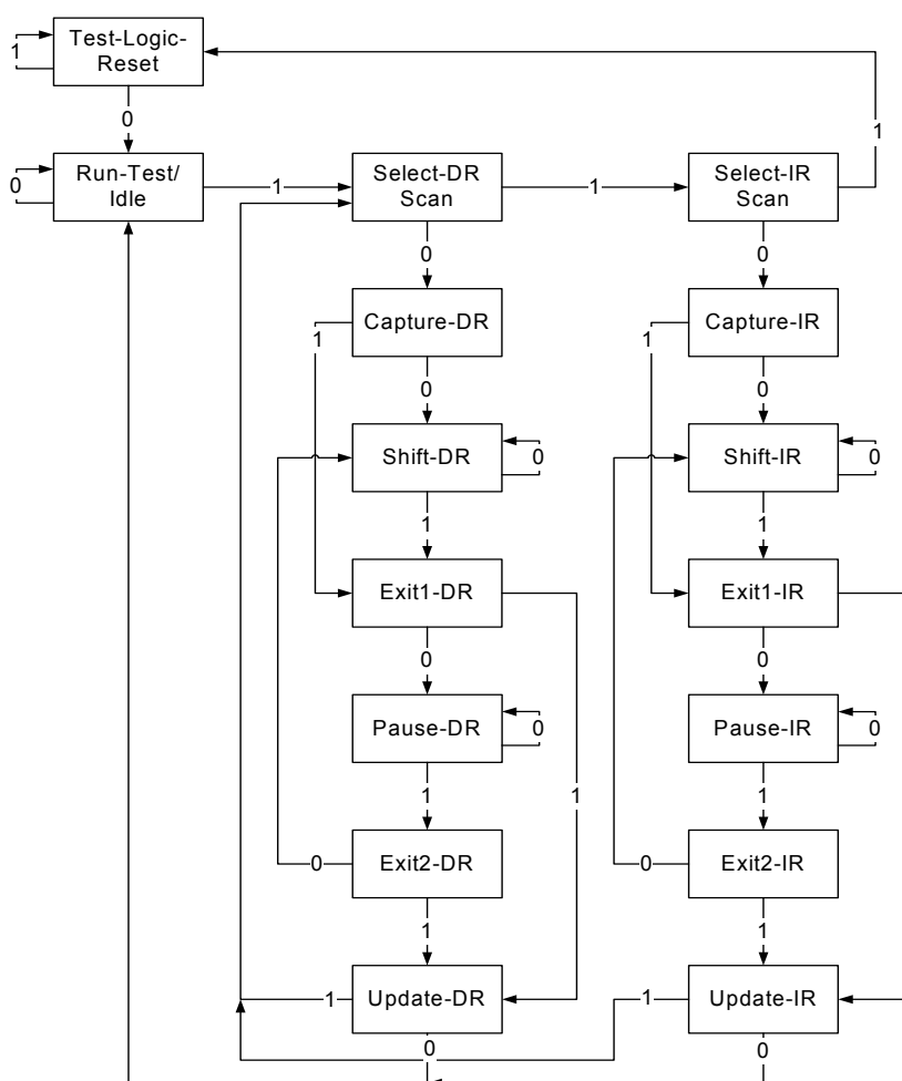
Figure 38-2. TAP Controller State Diagram
