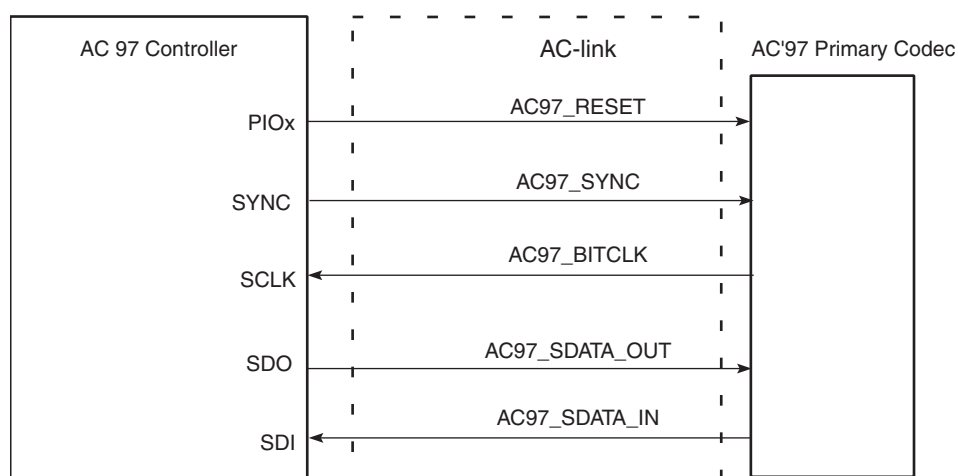
Figure 25-2. Application Block diagram
