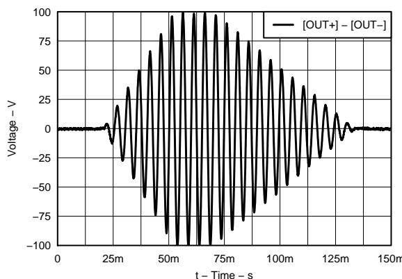
Figure 17. Example Waveform – Envelope Down
