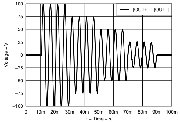
Figure 16. Example Waveform – Amplitude
