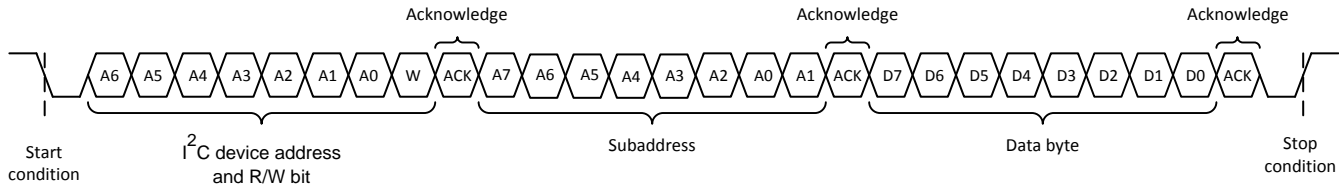
Figure 31. Single-Byte Write Transfer
