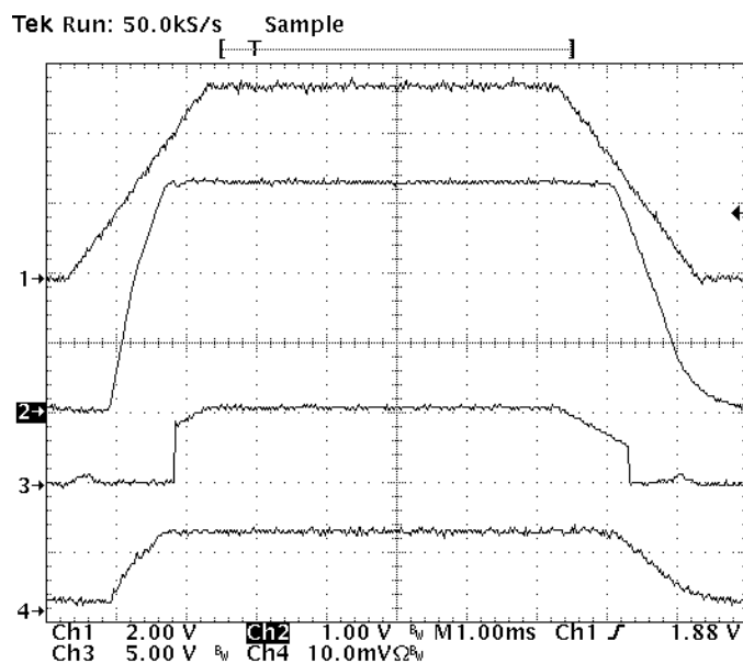
Figure 3–1. Input Voltage Ramp
