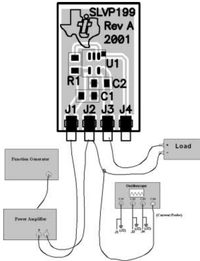
Figure 2–1. Recommended TPS79733EVM Test Setup
