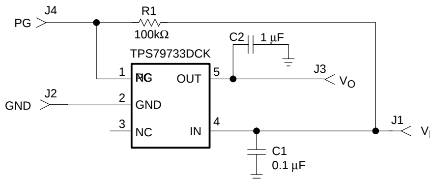
Figure 1–1. TPS79733EVM Schematic Diagram
