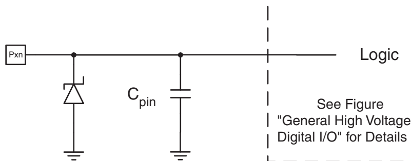
Figure 14-1. High Voltage I/O Pin Equivalent Schematic
