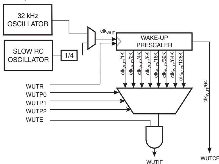
Figure 10-1. Wake-up Timer
