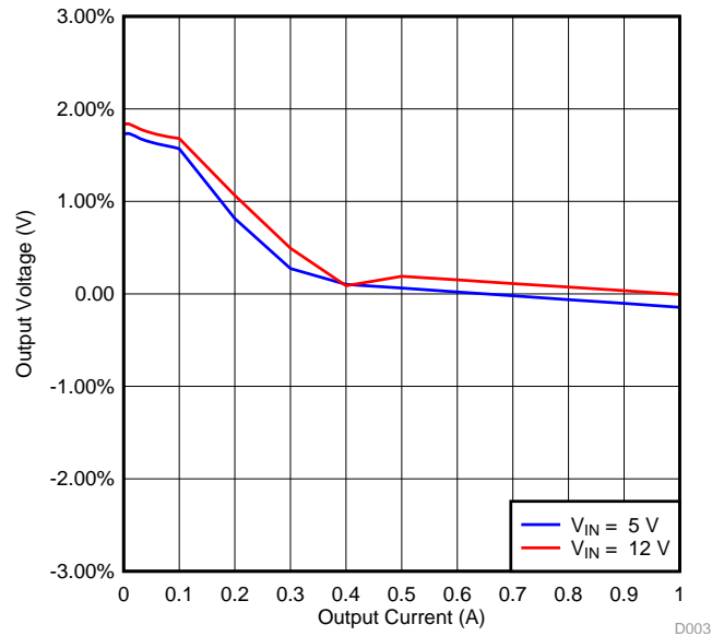
Figure 3. Load Regulation
