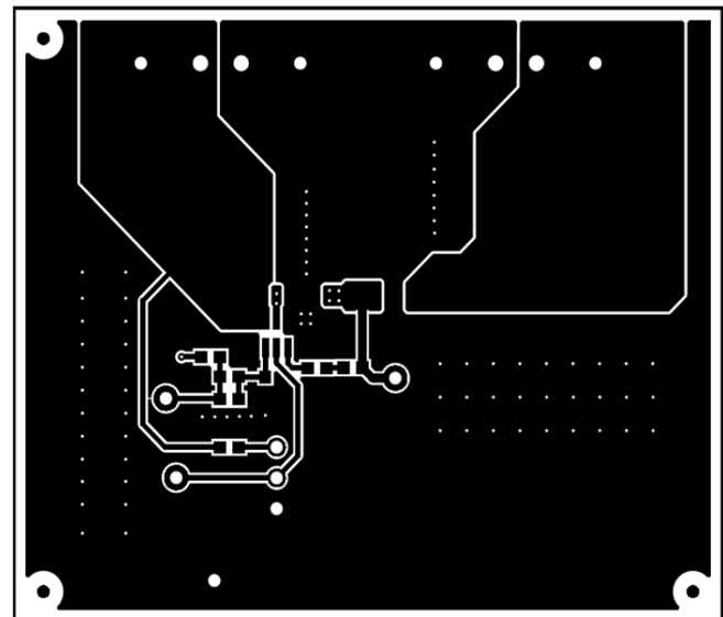
Figure 15. Top Layer
