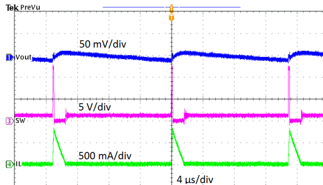
Figure 8. Output Voltage Ripple, I_{OUT} = 10\text{ mA}
