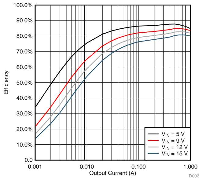
Figure 2. Light-Load Efficiency
