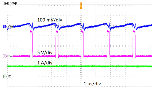
Figure 9. Input Voltage Ripple, I_{OUT} = 1\text{ A}
