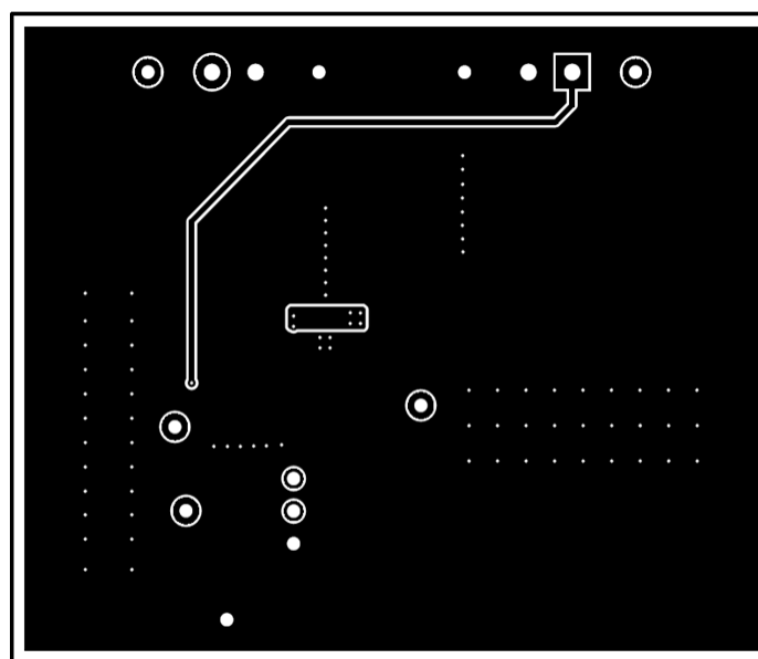
Figure 16. Bottom Layer
