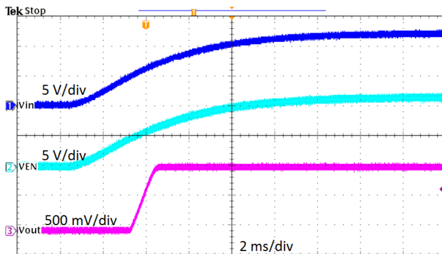
Figure 10. Start-Up Relative to Input Voltage
