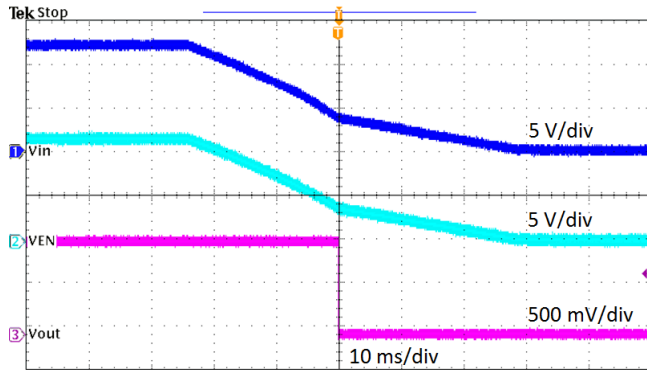
Figure 12. Shut-Down Relative to Input Voltage
