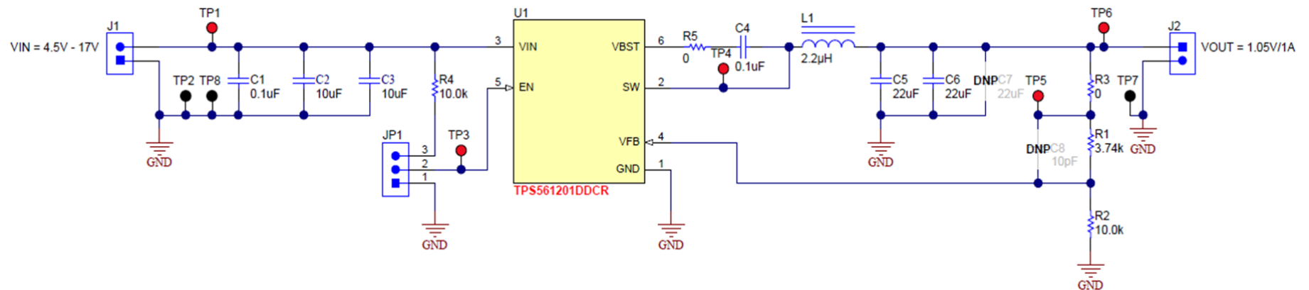
Figure 17. TPS561201EVM-896 Schematic Diagram
