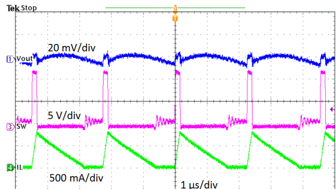
Figure 7. Output Voltage Ripple, I_{OUT} = 250\text{ mA}
