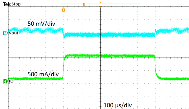
Figure 5. Load Transient Response, 10% to 100% Load Step
