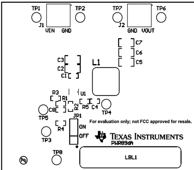
Figure 14. Top Assembly
