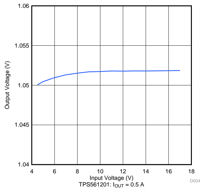
Figure 4. Line Regulation
