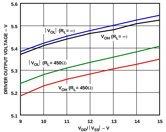
Figure 10. V_{OH}/V_{OL} vs. V_{DD}/V_{SS} (RS-232 Mode)
