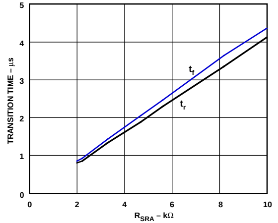
Figure 8. Typical Rise/Fall Times (RS-232 Mode) vs. R_{SRA}
