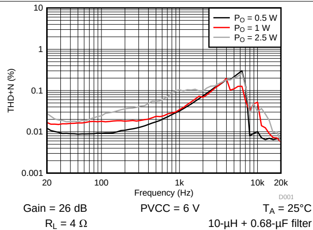
Figure 2. Total Harmonic Distortion + Noise (BTL) vs Frequency
