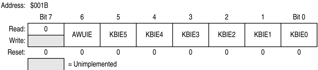
Figure 9-4. Keyboard Interrupt Enable Register (KBIER)
