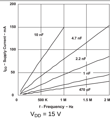
Figure 6. Supply Current vs Frequency
