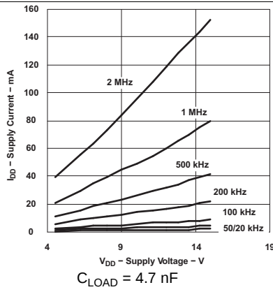
Figure 8. Supply Current vs Supply Voltage
