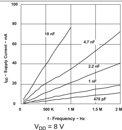
Figure 4. Supply Current vs Frequency
