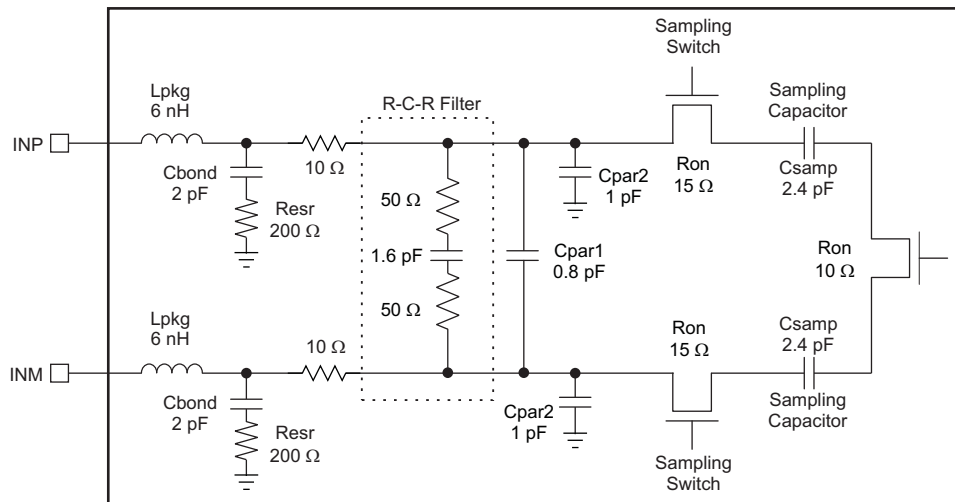
Figure 39. Input Stage
