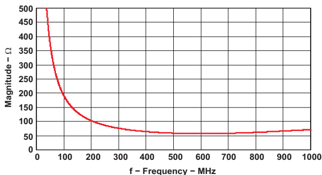
Figure 42. Input Impedance, Z_i
