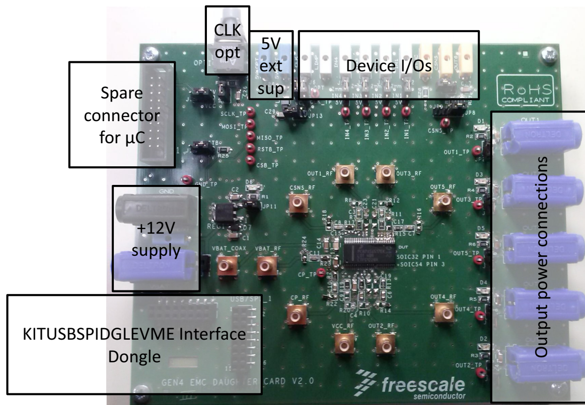
Figure 6. Connector Designations
