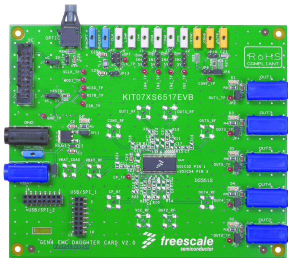
54-pin SOIC
