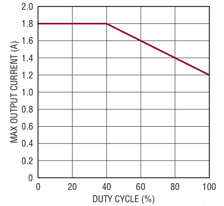
Channel 3/Channel 4 Maximum Output Current vs Duty Cycle
