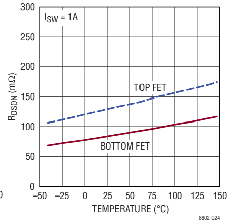
Channel 3/Channel 4 R_{DS(on)} vs Temperature
