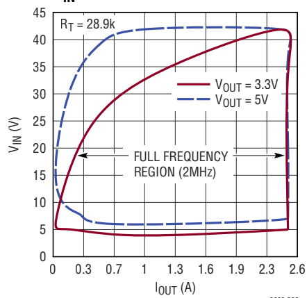
Channel 2 Full Frequency V_{IN} vs Load Current
