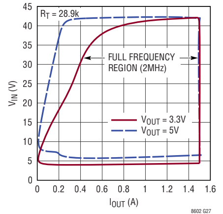
Channel 1 Full Frequency V_{IN} vs Load Current
