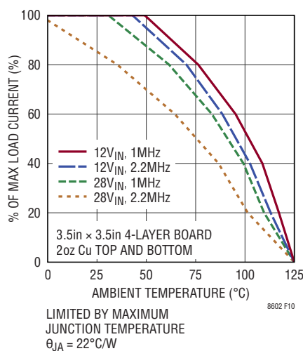
Figure 10. Thermal Derating, I-Grade
