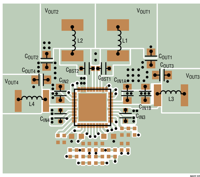
Figure 9. Recommended QFN Package PCB Layout
