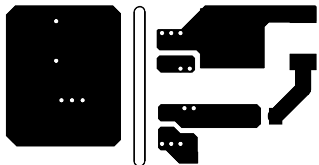
Figure 44. Bottom Layer Traces and Copper
