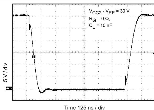
Figure 26. Output Waveform
