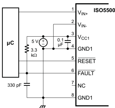
Figure 63. FAULT Pin Circuitry for High CMTI
