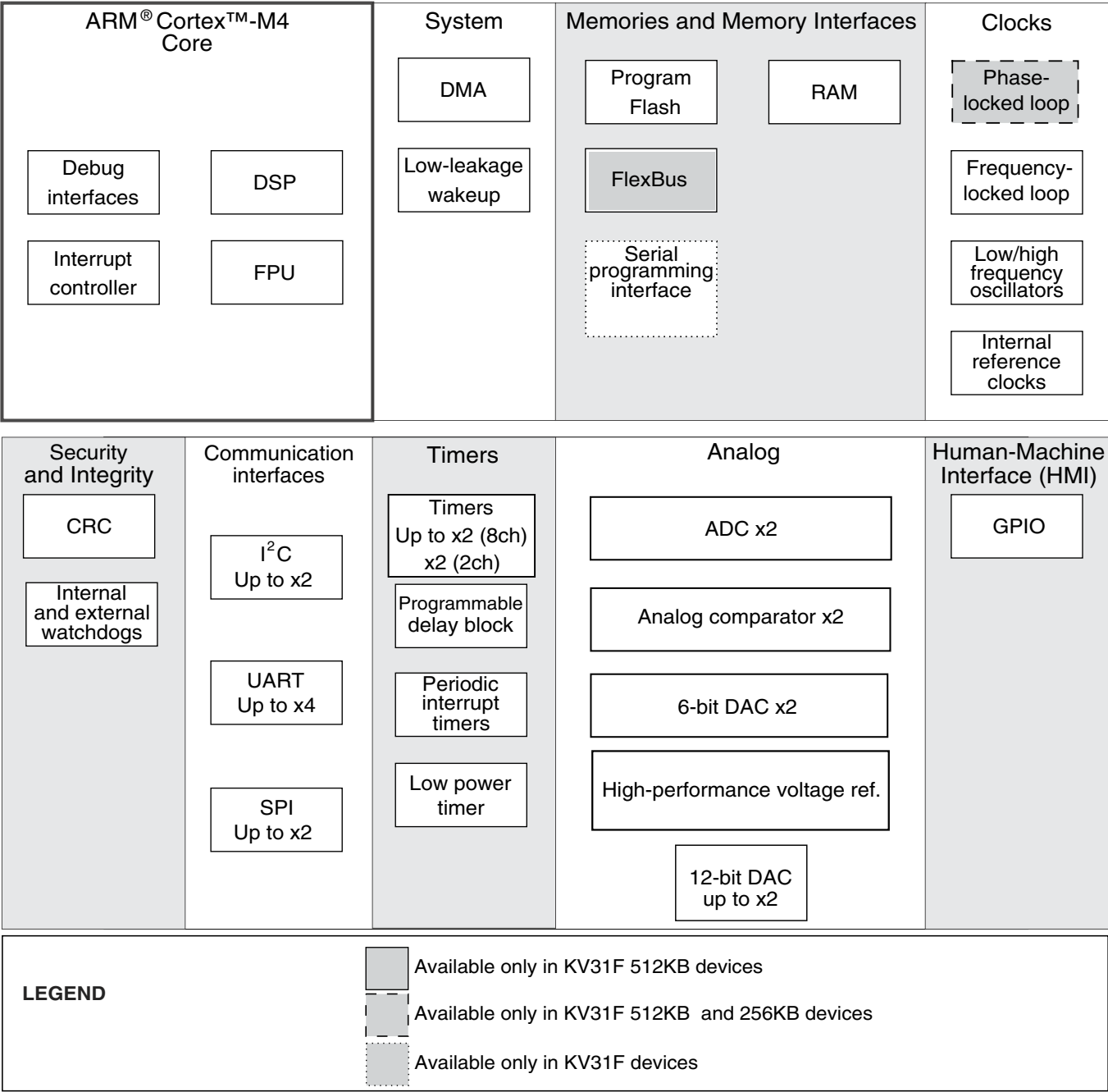
Figure 1. KV30F/KV31F block digram
