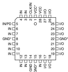
Figure 1-5. PLCC
