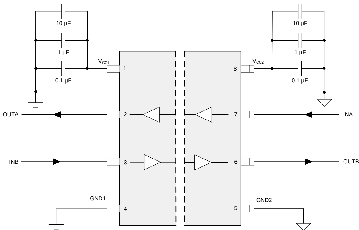
Figure 3. ISO7721/ISO7021 EVM Configuration
