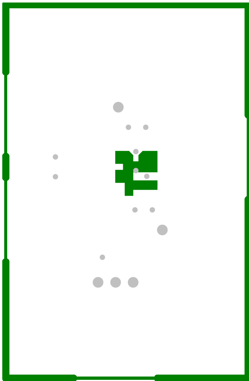
Figure 3. OPA838DBVEVM Layer 2
