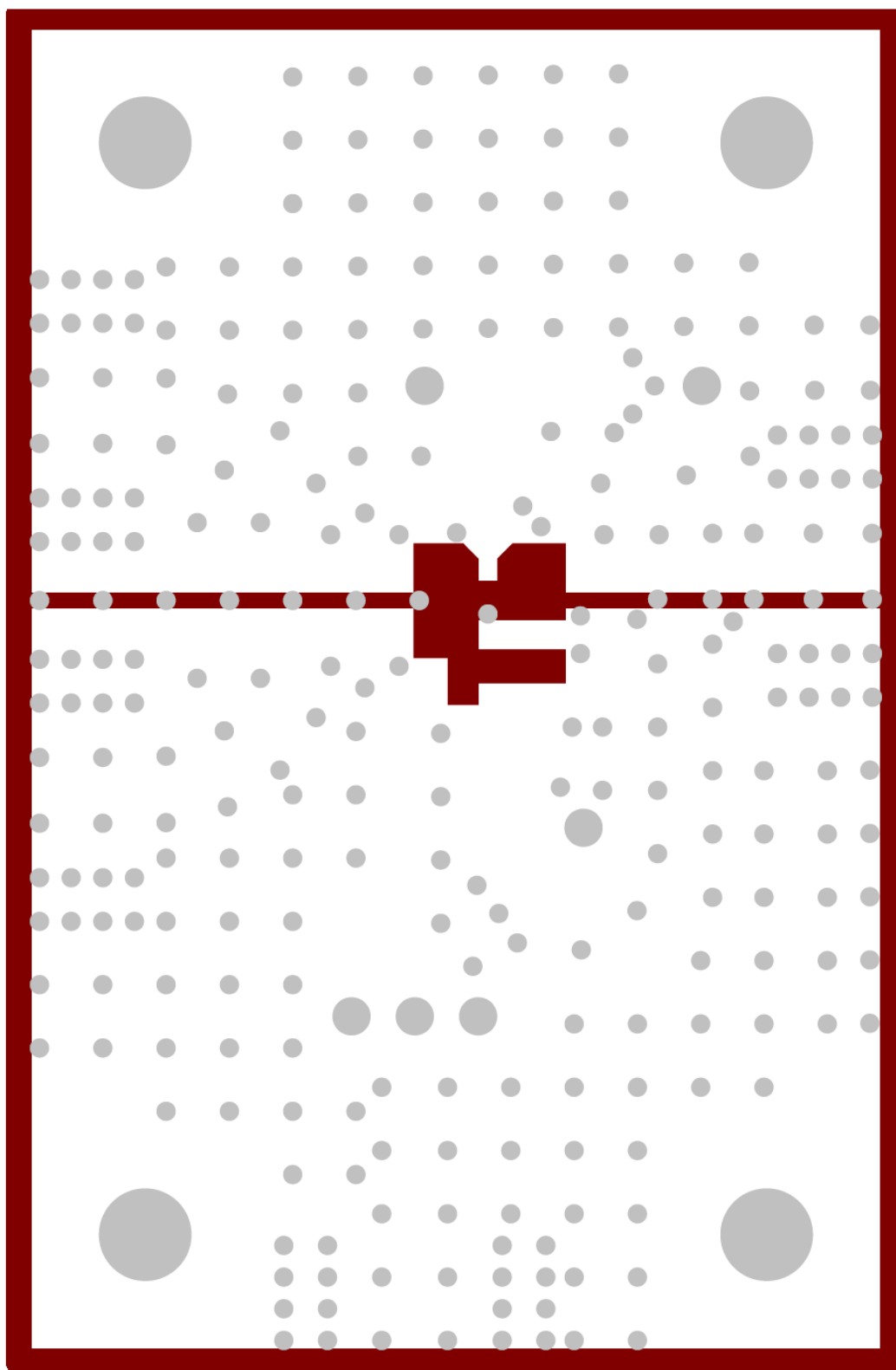
Figure 4. OPA838DBVEVM Layer 3
