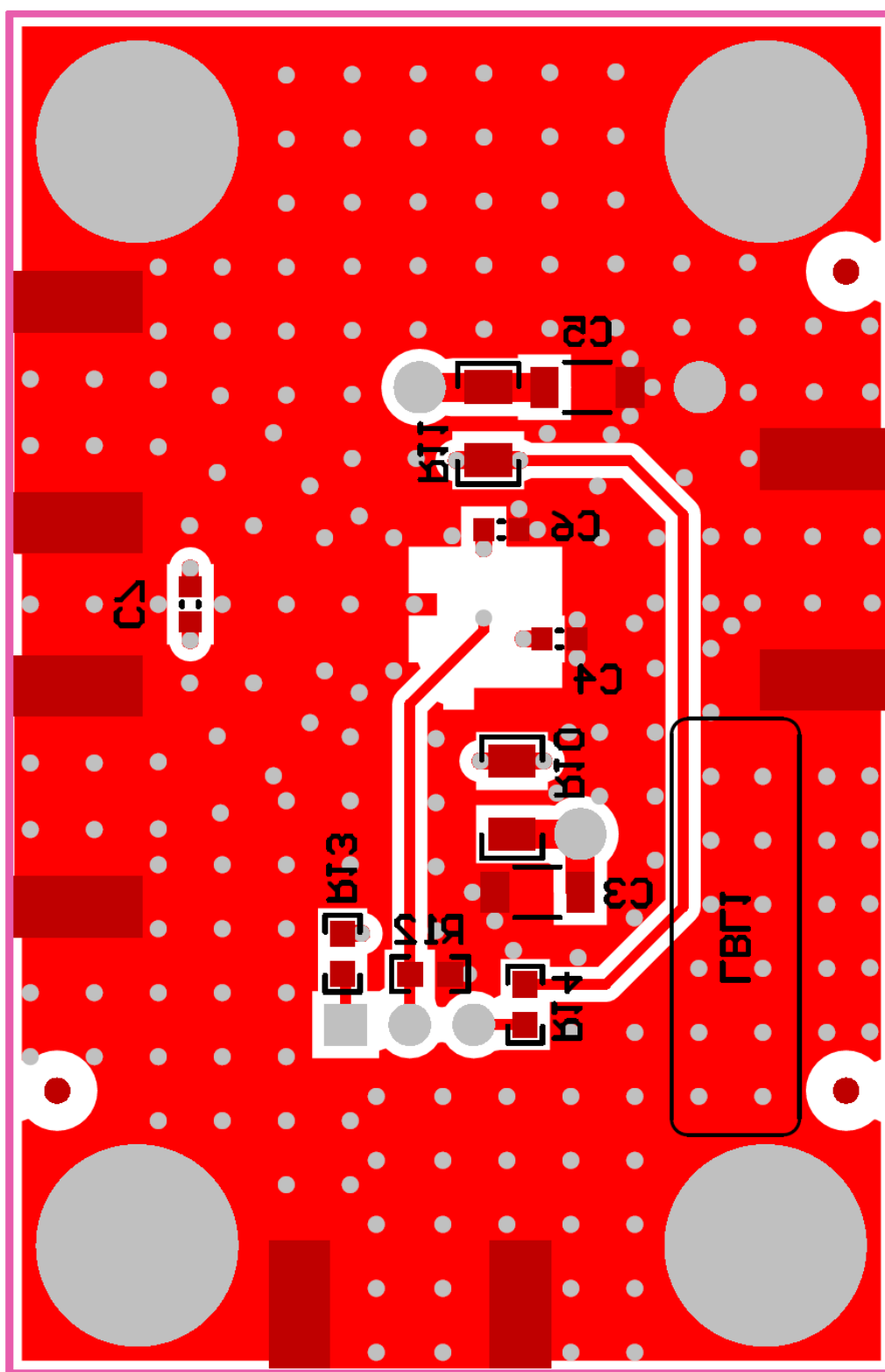
Figure 5. OPA838DBVEVM Bottom Layer
