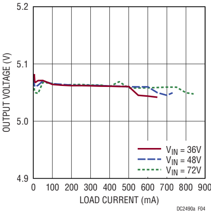
Figure 4. Load and Line Regulation
