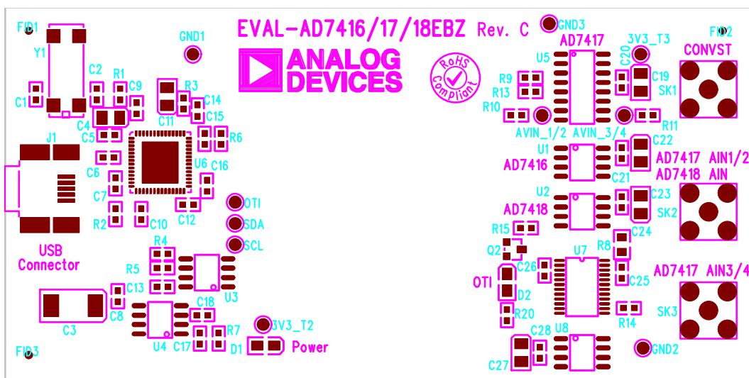
Figure 19. EVAL-AD7416/7/8EBZ Board—Silkscreen
