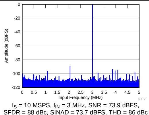
Figure 139. FFT for 10-MSPS Sampling Speed
