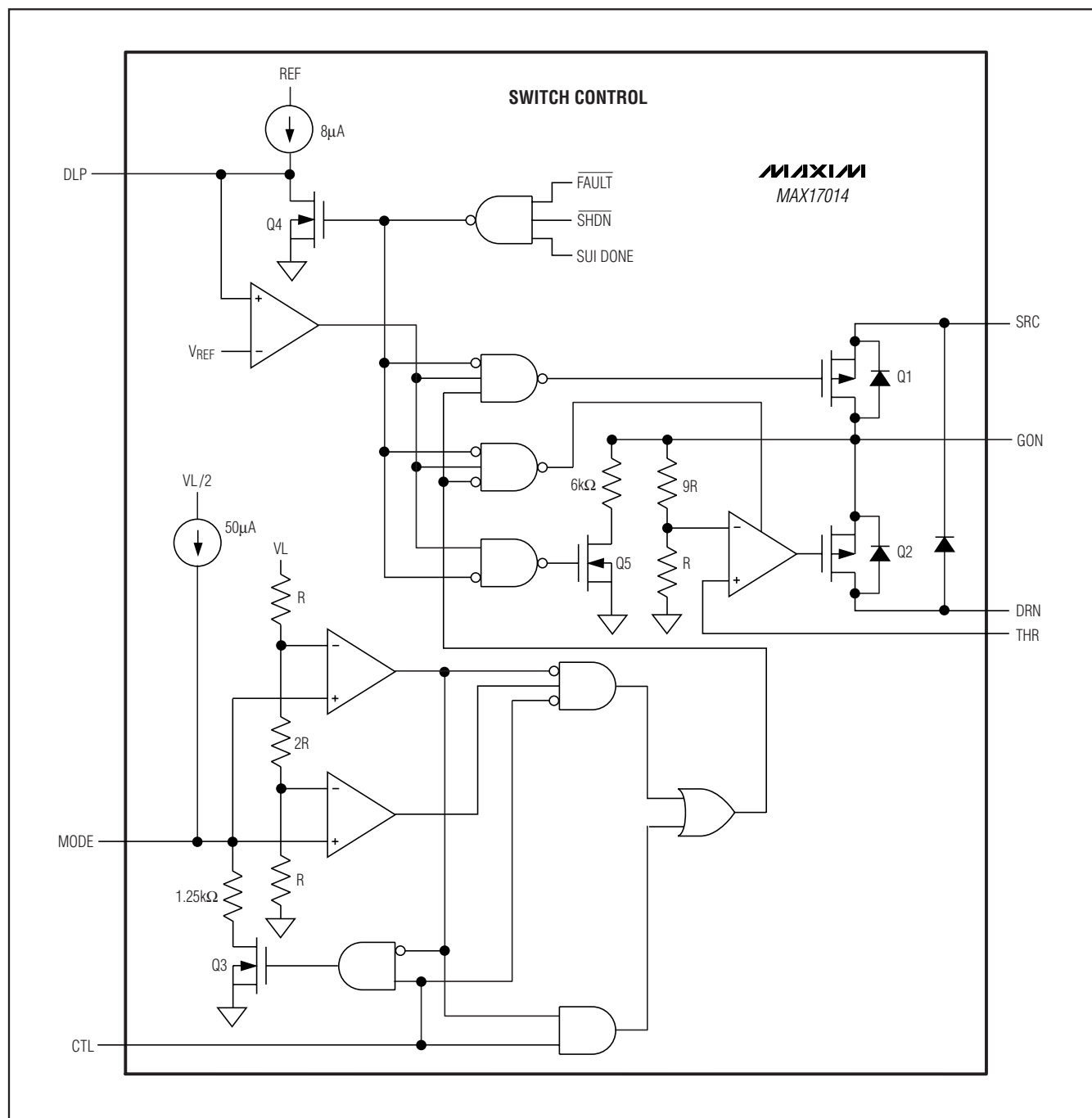
Figure 5. Switch Control
