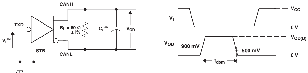
Figure 10. t_{\text{LOOP}} Test Circuit and Waveforms
