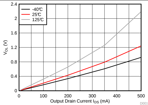
Figure 1. V_{OL} ( V_{DS} )
