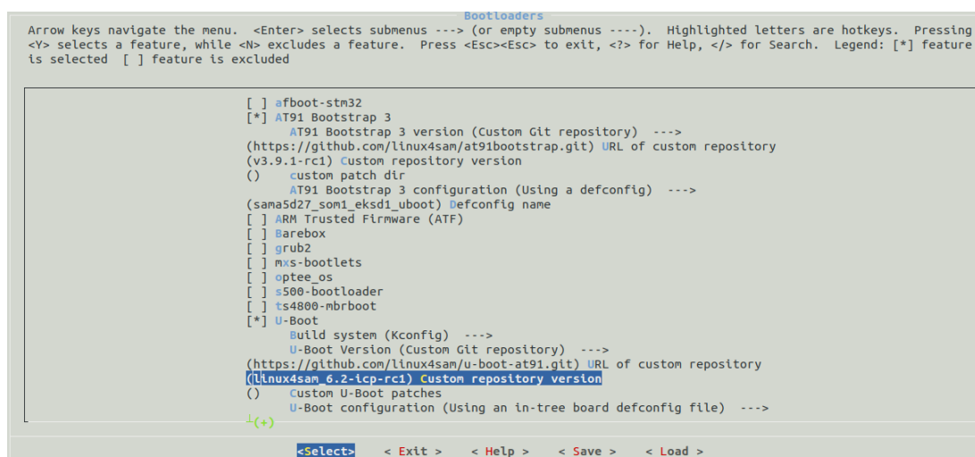
Figure 5-6. U-boot Repository Version
