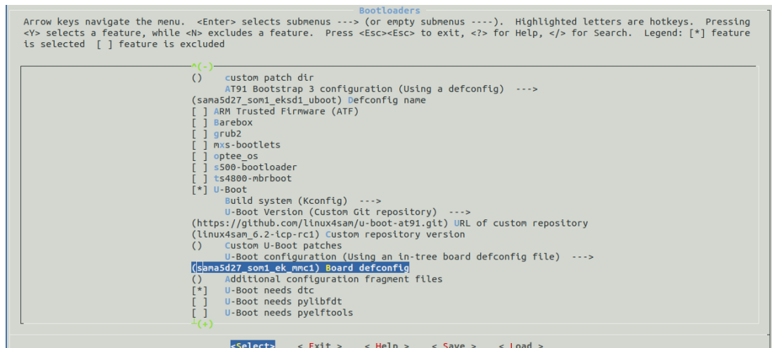
Figure 5-8. U-Boot defconfig
