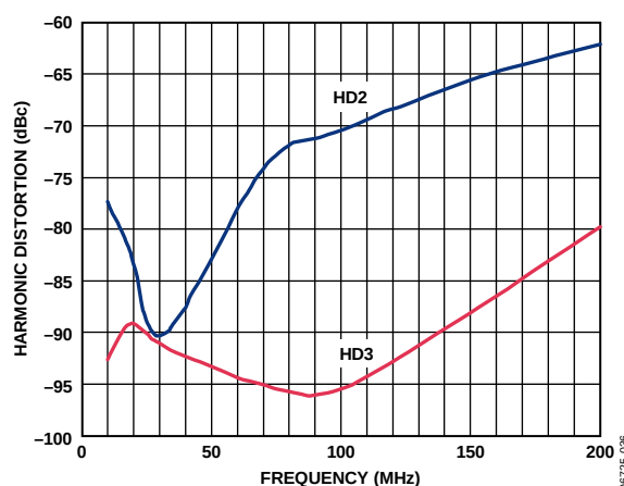
Figure 35. Harmonic Distortion vs. Frequency of Single-Ended-to-Differential Conversion
