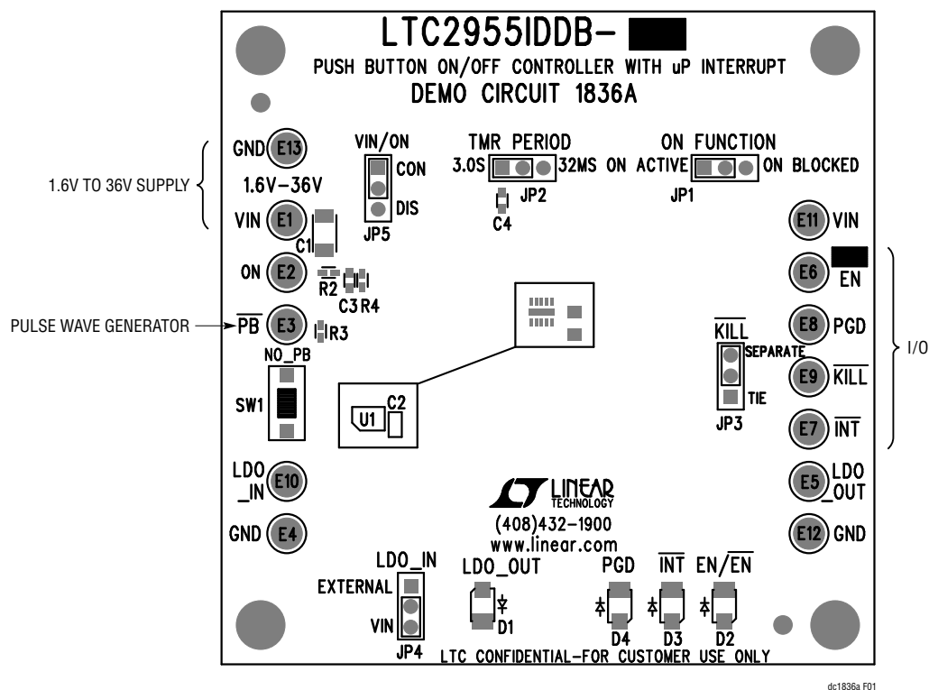
Figure 1. Proper Test Equipment Setup
