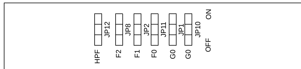
FIGURE 2-7: MCP3905A Jumper Selections.
