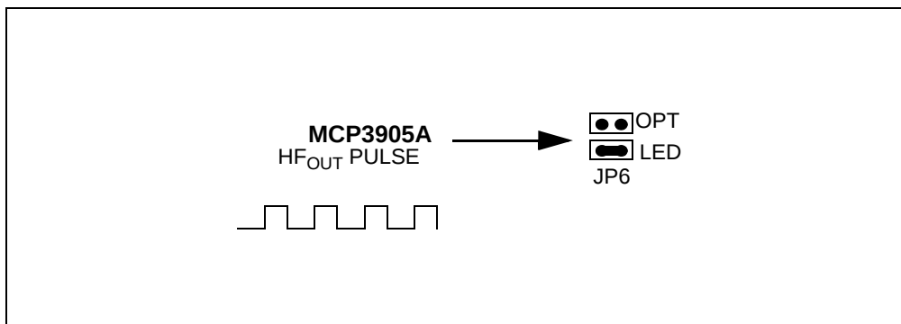
FIGURE 2-5: Connecting the MCP3905A High-Frequency Output to the LED.
