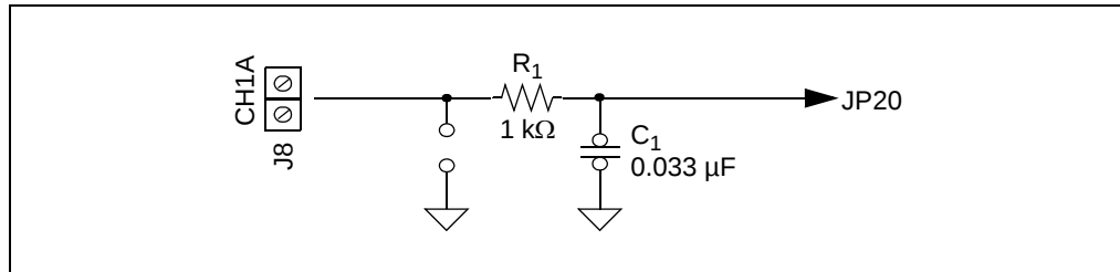
FIGURE 2-10: Channel 1 RC Circuit A.
