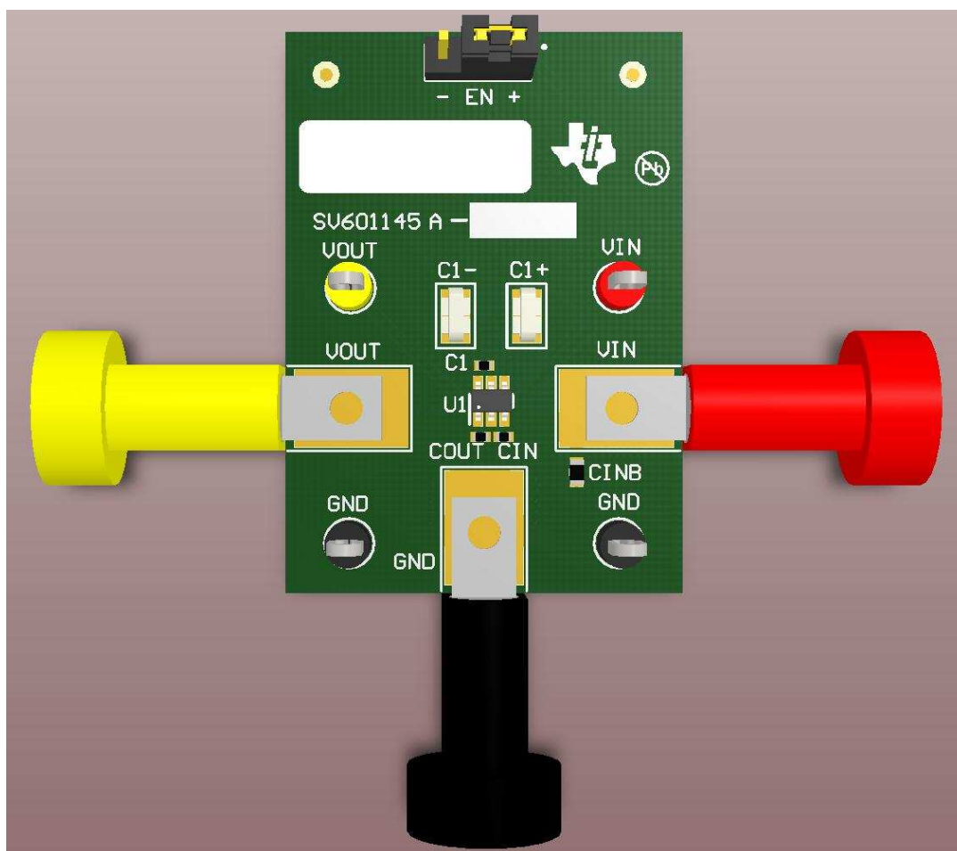
Figure 2. Jumper Configuration
