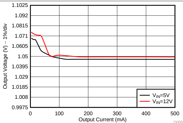
Figure 10. Load Regulation
