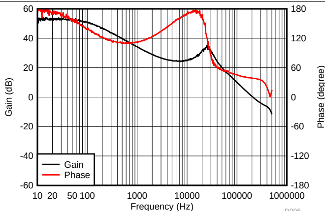
Figure 12. Loop Response, I_{\text{OUT}} = 0.25\text{ A}
