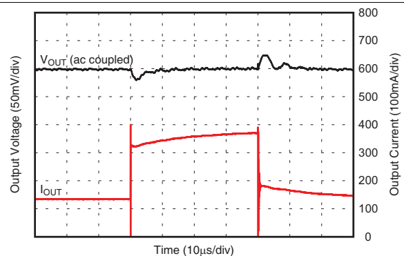
Figure 13. Transient Response, 25% to 75% Load Step
