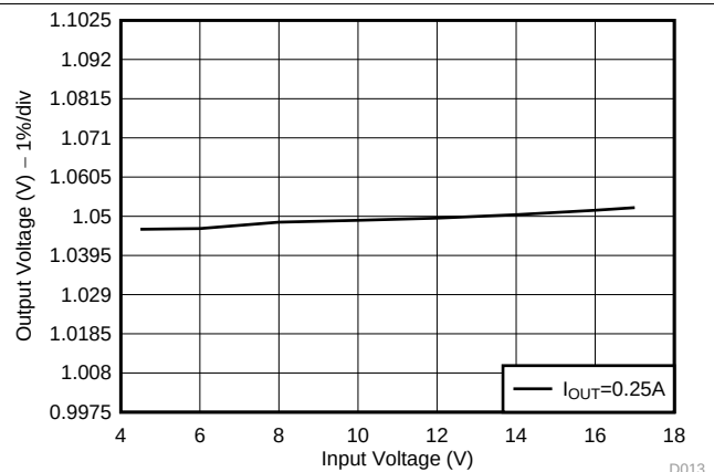
Figure 11. Line Regulation
