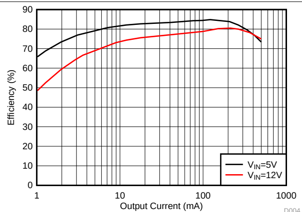
Figure 9. Light-Load Efficiency
