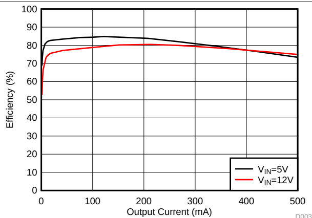
Figure 8. Efficiency
