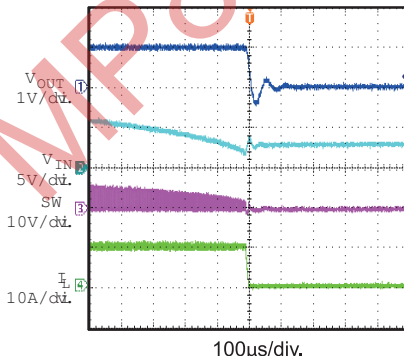
Shutdown Through I_{IN} I_{OUT}=10A
