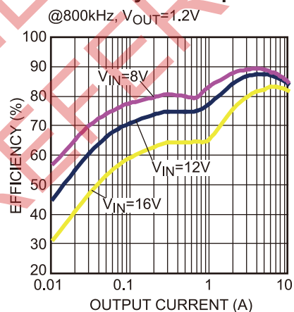
Figure 30 — Efficiency Curve
