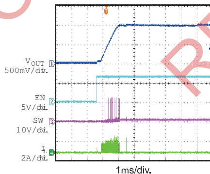
Start up through EN I_{OUT}=0
