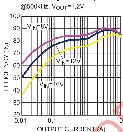
Figure 28 — Efficiency Curve
