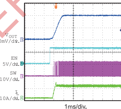
Start up through EN I_{OUT}=10A
