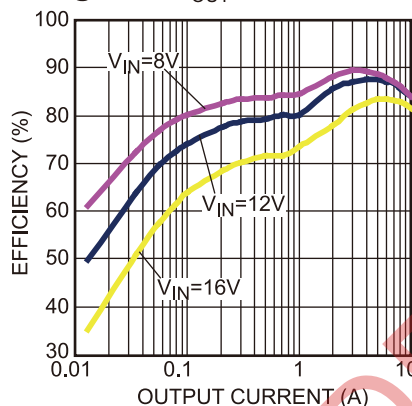
Figure 16 — Efficiency Curve
