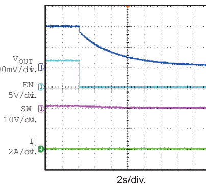
Shutdown Through EN I_{OUT}=0
